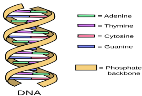
Figure 1. Structure of DNA
