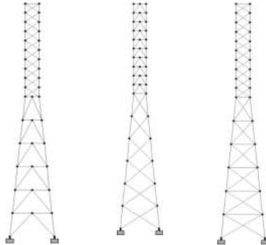
Figure 2.0 geometry of the Model 1: (K-XX), Model 2: (XX-K), Model 3: (XB-XX) tower respectively.
